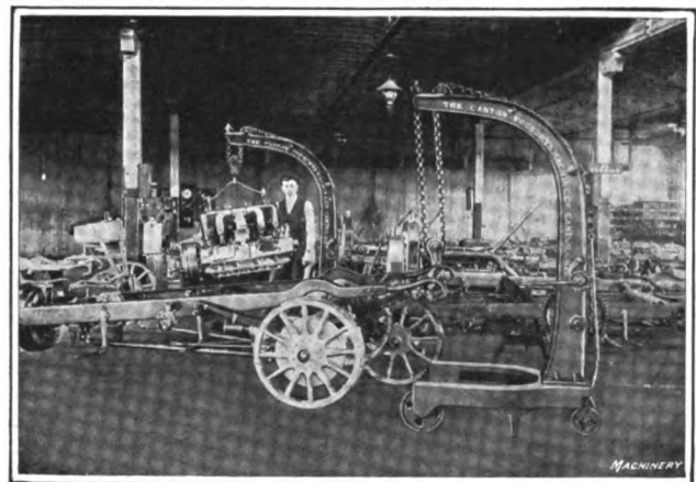
Fig. 2—Portable cranes are used for many purposes. Their chief field is for lifting work in confined spaces that cannot be served by traveling cranes or trolleys. They can also be used to advantage where there is not enough work to warrant installing a crane or trolley system. Canton Foundry & Machine Co.'s portable cranes are shown in use in a garage.
